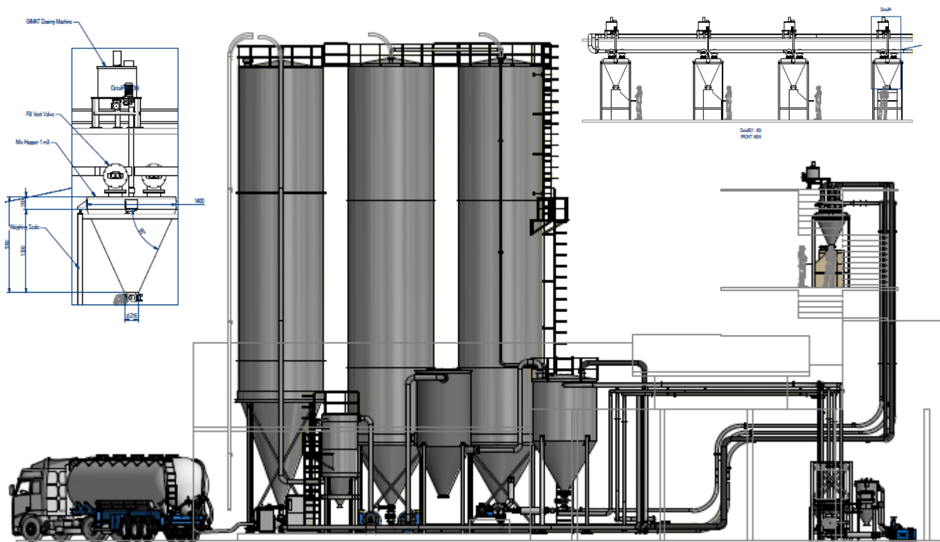
Silos Weighting system (PVC powder & Calcium Carbonate Powder ) Saha Area , Twin Lion brand PVC pipe factory
