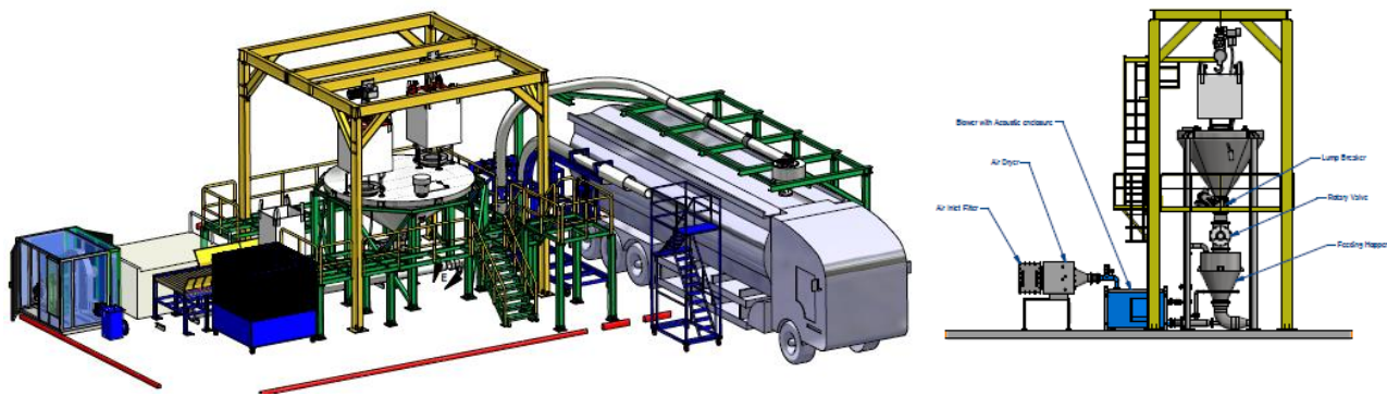
Sea bulk Loader or Bulk Truck loader / Mobile or Fixed Station
