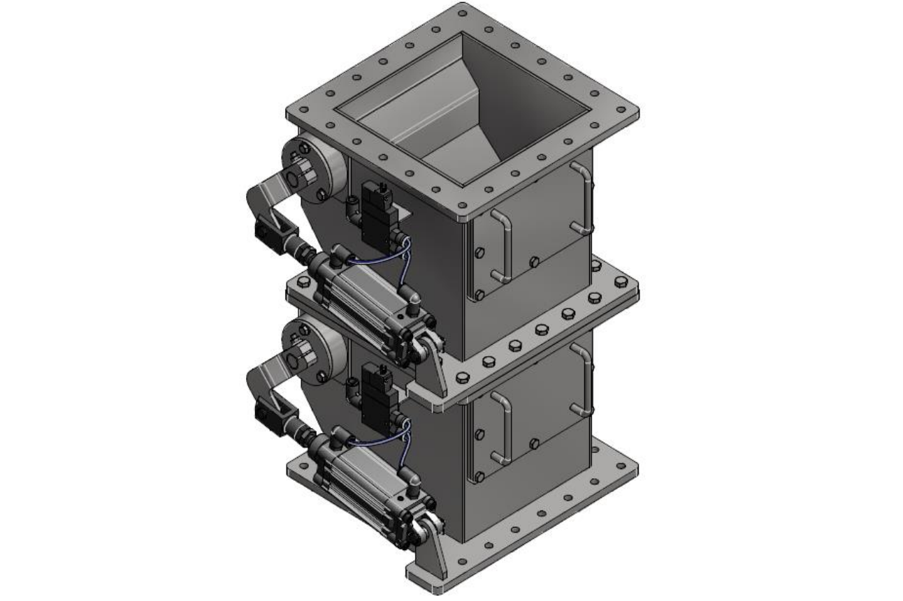
DOUBLE FLAP VALVE
